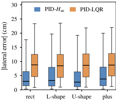
(a) sweep lateral error
