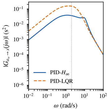
(c) linear disturbance gain
